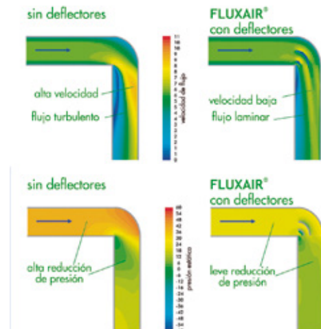
CODO VERTICAL
